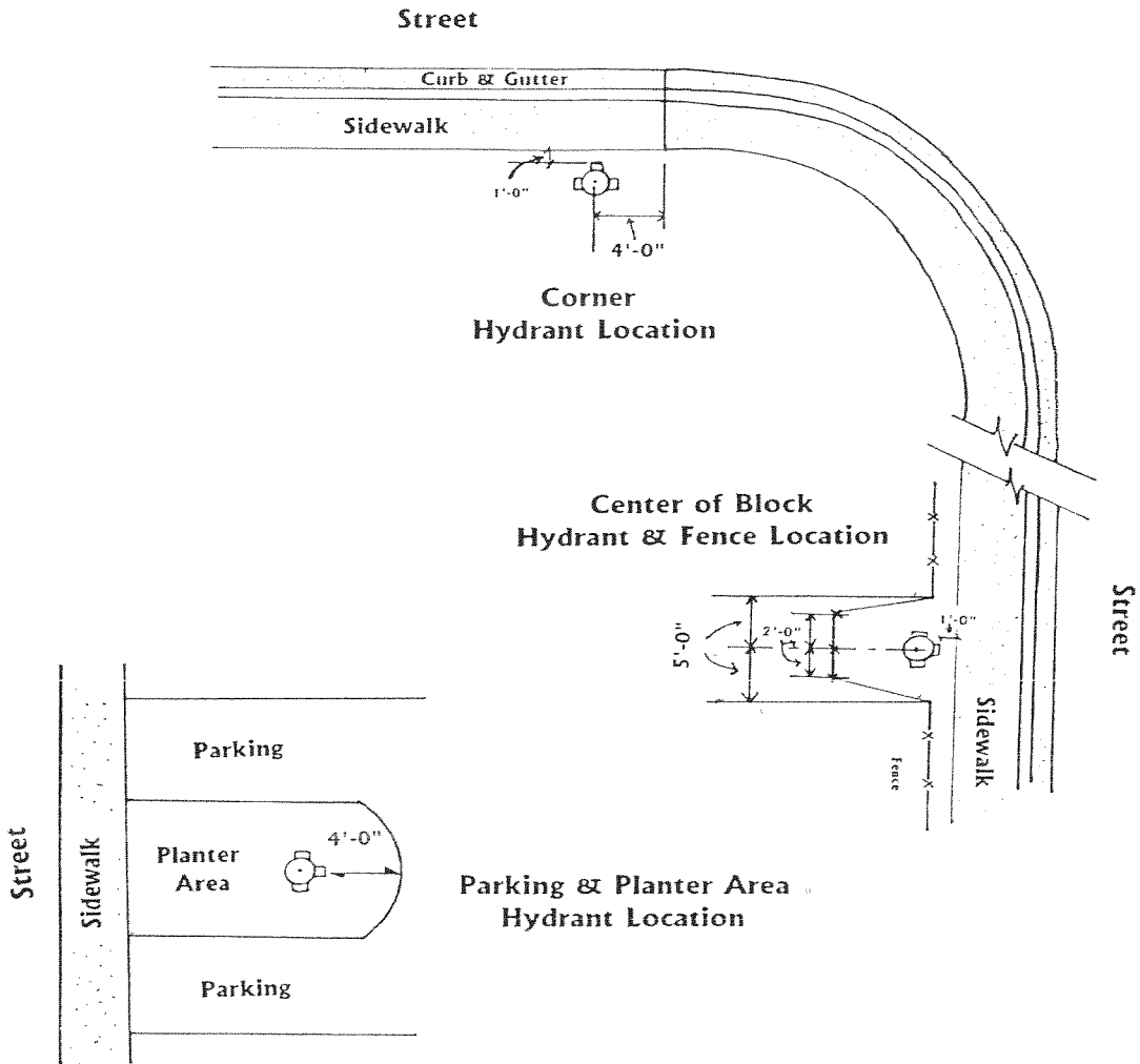
Standard Fence & Hydrant Locations
